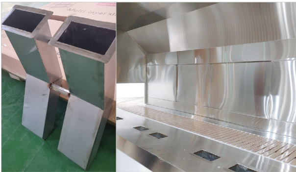
08. 벽체 STS마감(STS WALL FINISH)
